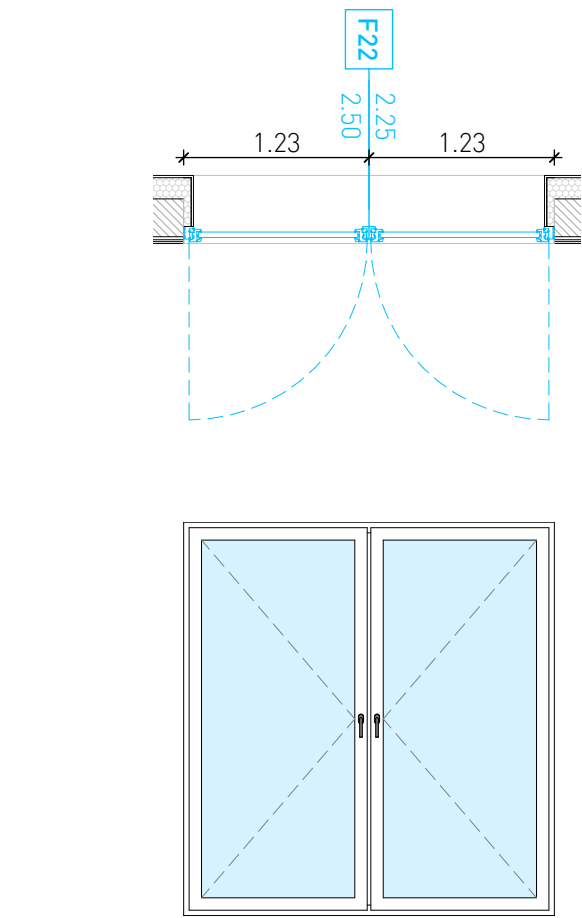
F22: PORTAFINESTRA 225*250
