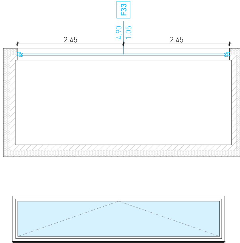
F33: LUCERNARIO 490*105
