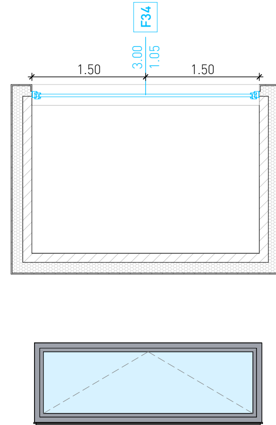
F34: LUCERNARIO 300*105
