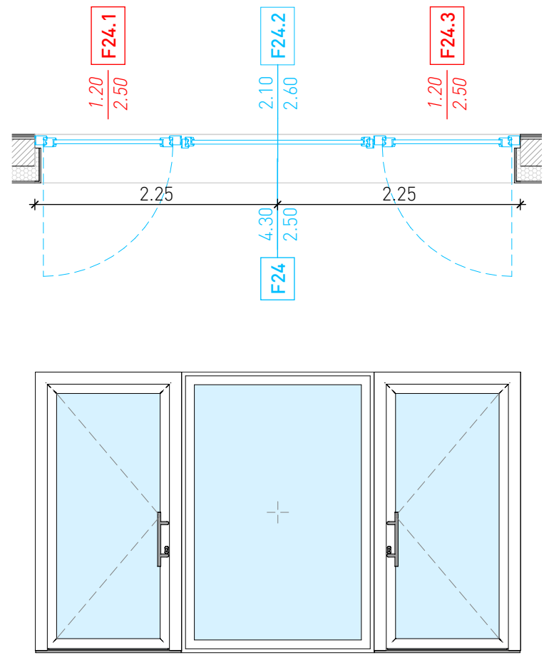
F24: PORTAFINESTRA 430*250
