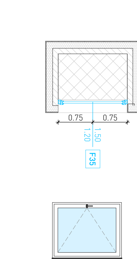
F35: LUCERNARIO 150*120
