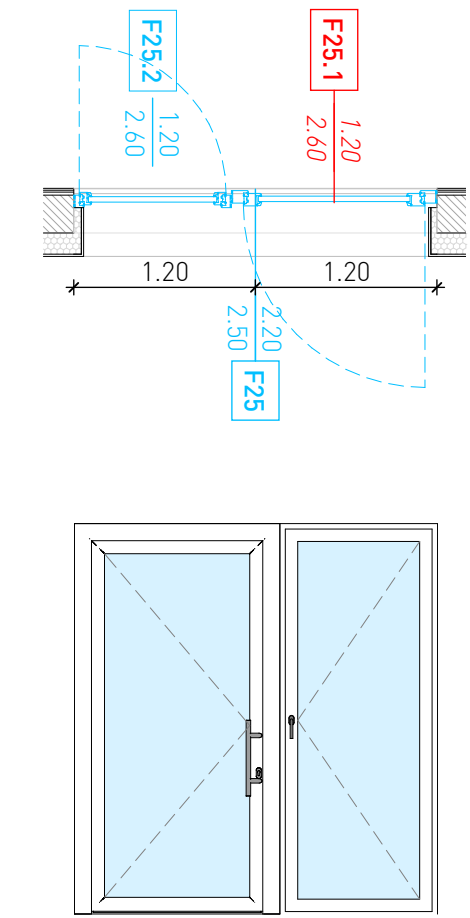
F25: PORTAFINESTRA 220*250
