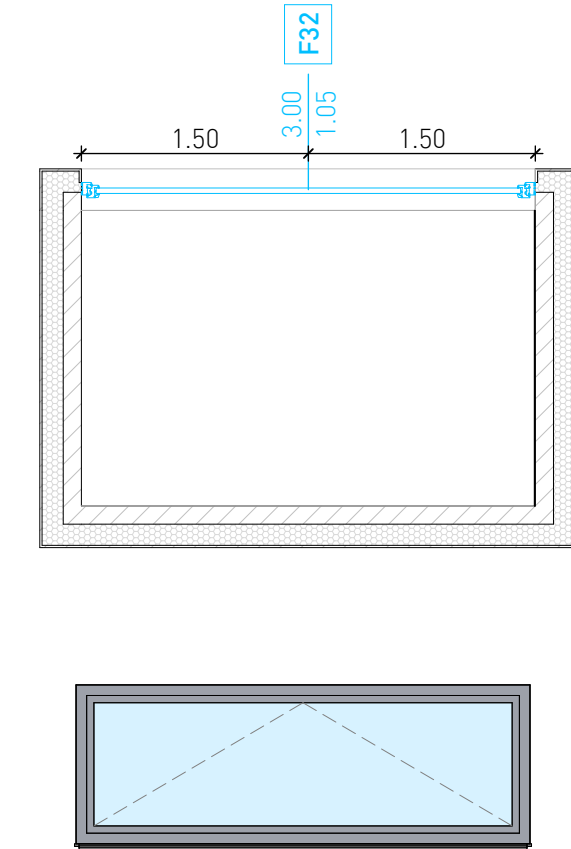
F32: LUCERNARIO 300*105
