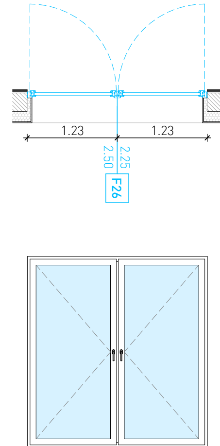
F26: PORTAFINESTRA 225*250
