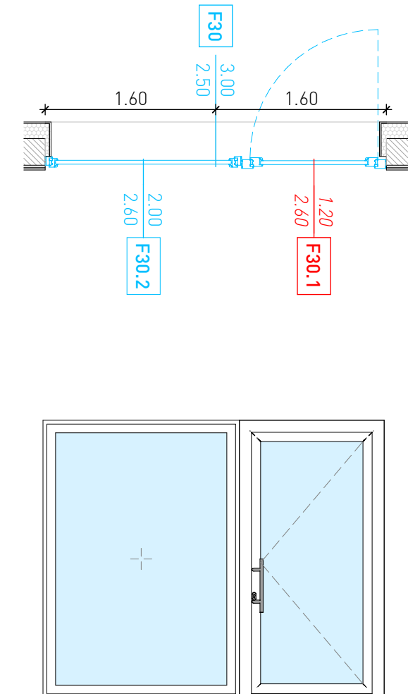
F30: PORTAFINESTRA 300*250
