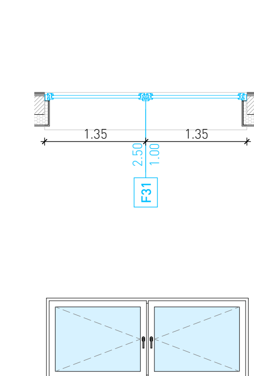
F31: FINESTRA 250*100
